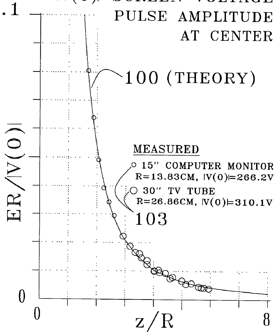
ELECTRIC FIELD AT A DISTANCE z FROM CRT SCREEN ON CENTER LINE
